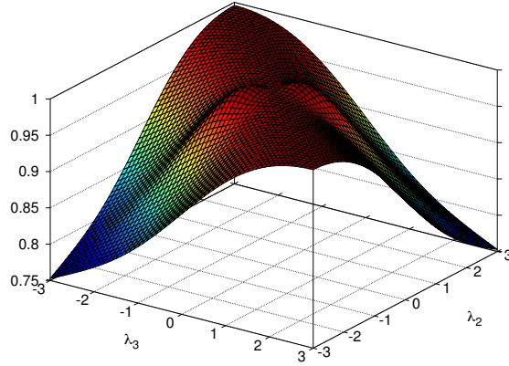
Figure 4: MSFE of optimal weights relative to standard weights when states are uncertain
