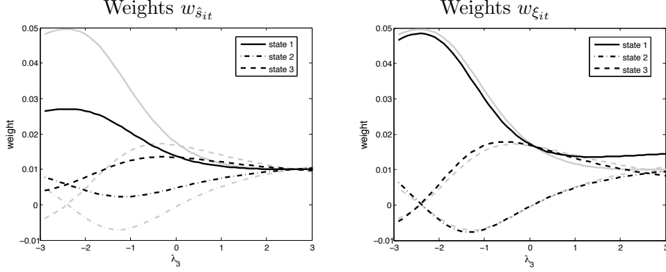
Figure 3: Optimal weights for a three state Markov switching model
